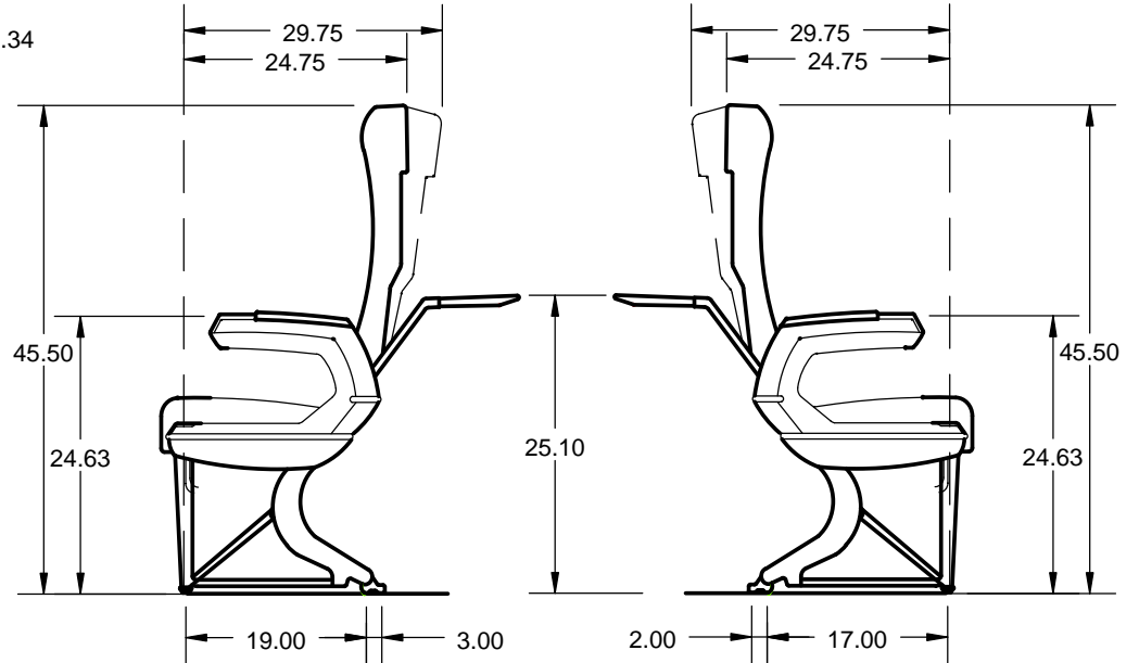
INBOARD VIEW
